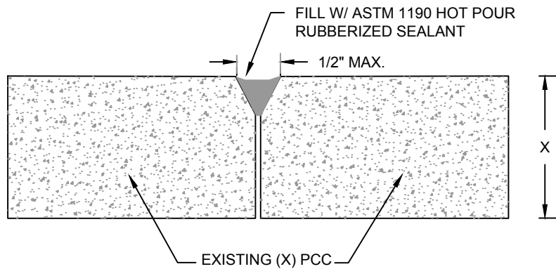
JOINT AND RANDOM CRACK ( 1/2" Wide or Less )
