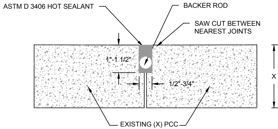
SAW AND SEAL ( Random Crack > 1/2" Width )
