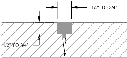
(C) STANDARD RESERVOIR-AND-FLUSH
