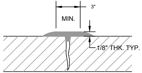
(B) SIMPLE OVERBAND
