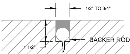
(E) DEEP RESERVOIR-AND-FLUSH (backer rod)
