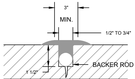
(F) DEEP RECESSED OVERBAND (backer rod)
