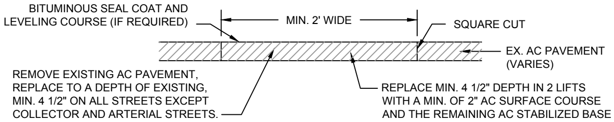
AC PAVEMENT FAILURE
