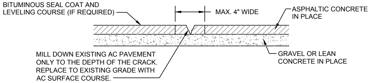
TYPICAL JOINT FAILURE REPAIR
