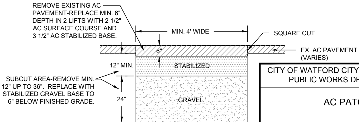
SUB-BASE FAILURE
