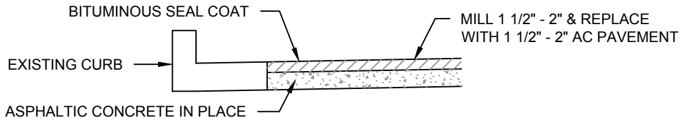
TYPICAL MILL & OVERLAY DETAIL
