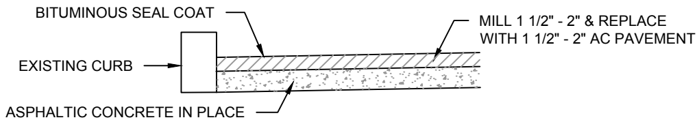
TYPICAL MILL & OVERLAY DETAIL
