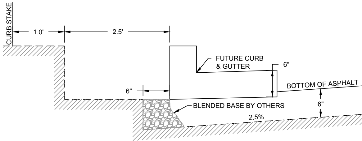
TYPICAL CURB GRADING SECTION
