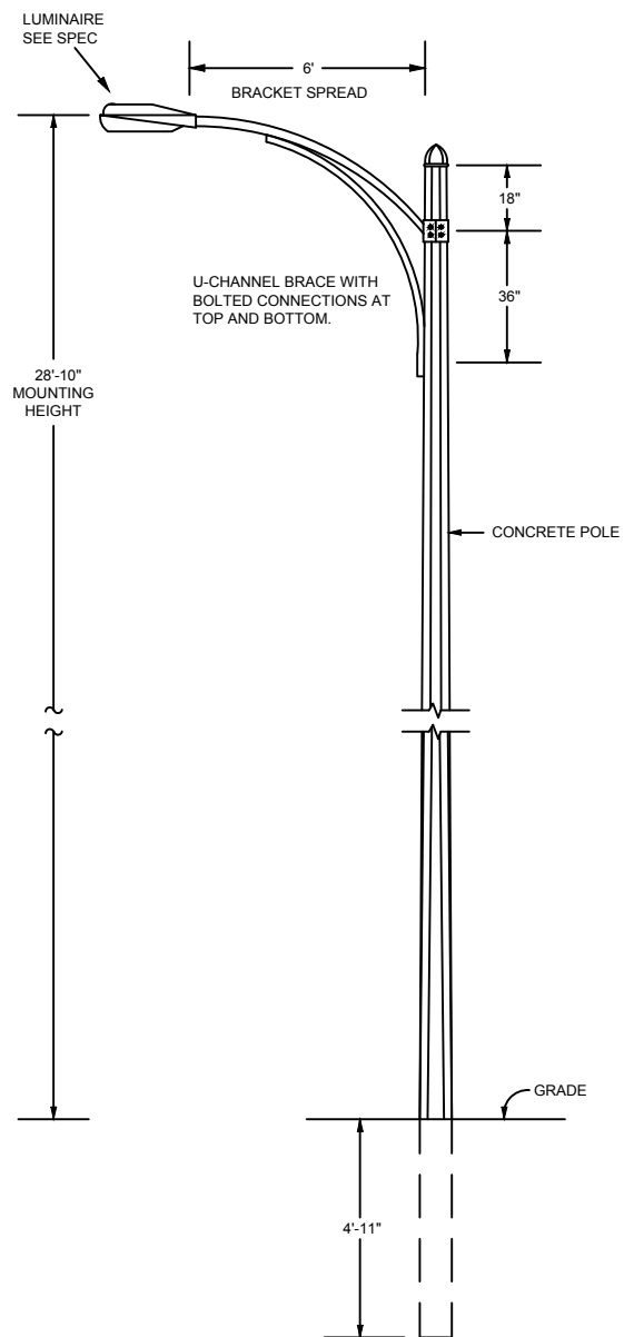
TYPE L & L1 POLE DETAIL NO SCALE
